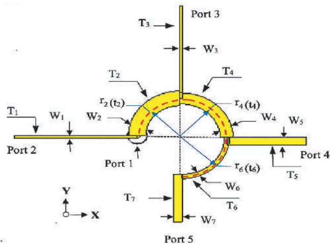
FIGURE 1. The SSFN configuration.
